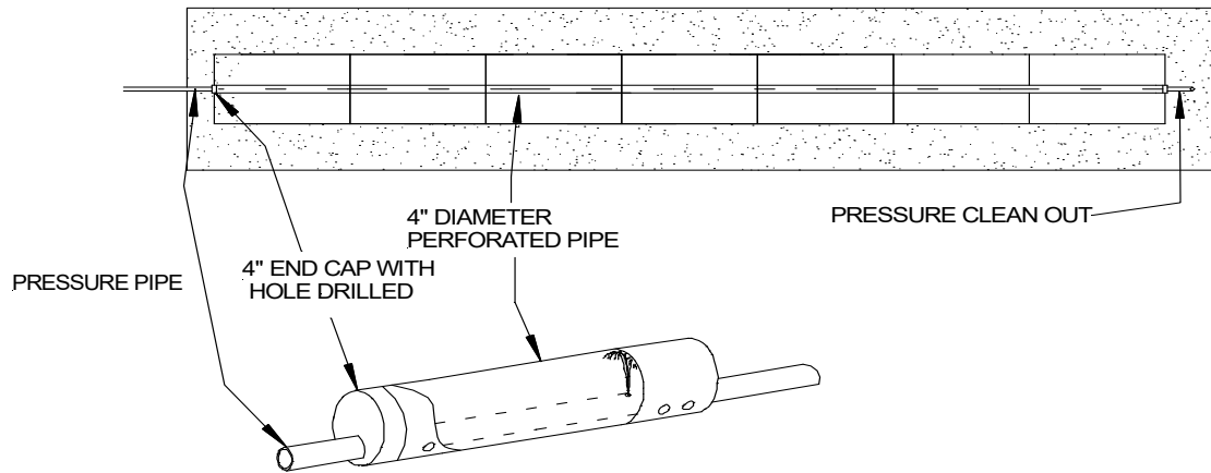
FIGURE 10: PRESSURE PIPE PLACEMENT
