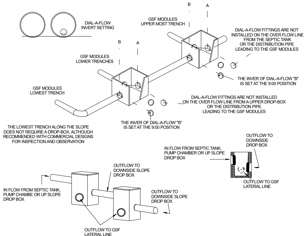
FIGURE 4: SEQUENTIAL DISTRIBUTION DROP-BOX DETAIL
