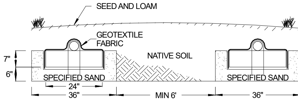
FIGURE 6: SECTION VIEW – TRENCH SYSTEM EXAMPLE – LEVEL SITE
