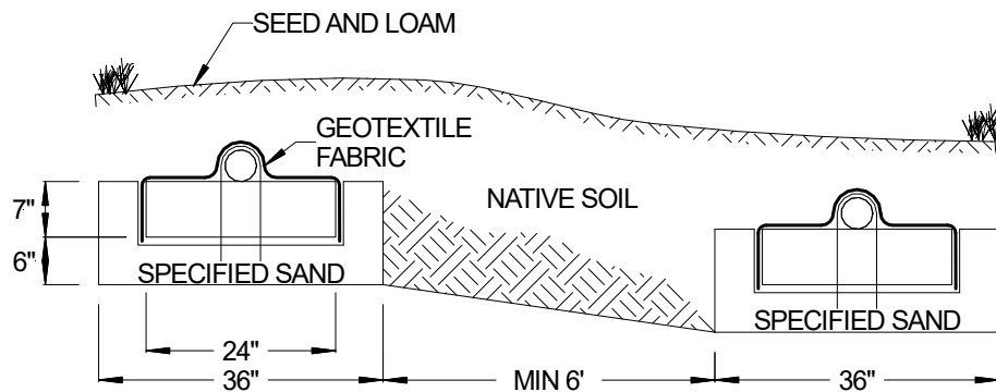
FIGURE 7: SECTION VIEW – TRENCH SYSTEM – SLOPING SITE
