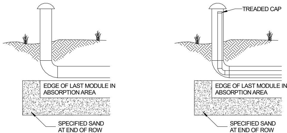
FIGURE 13: VENT LAYOUTS FOR GRAVITY AND LOW-PRESSURE SYSTEMS
