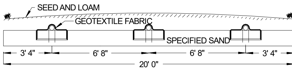
FIGURE 9: SECTION VIEW – BED SYSTEM EXAMPLE
