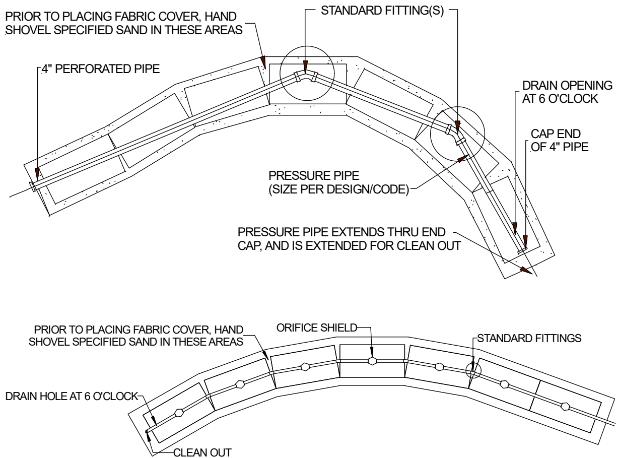
FIGURE 12: CONTOURED BED PRESSURE DISTRIBUTION
