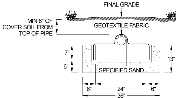
FIGURE 2: TYPICAL A42 CROSS SECTION
