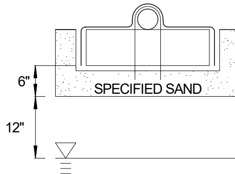
FIGURE 3: VERTICAL SEPARATION DISTANCE
