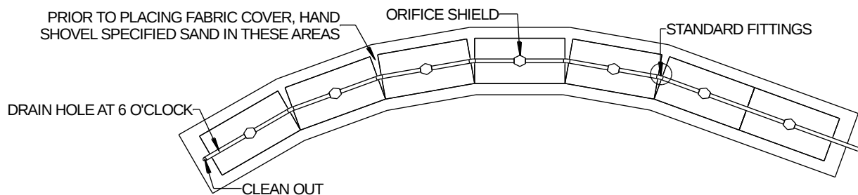
FIGURE 16: CONTOURED TRENCH PRESSURE DISTRIBUTION USING ORIFICE SHIELDS
