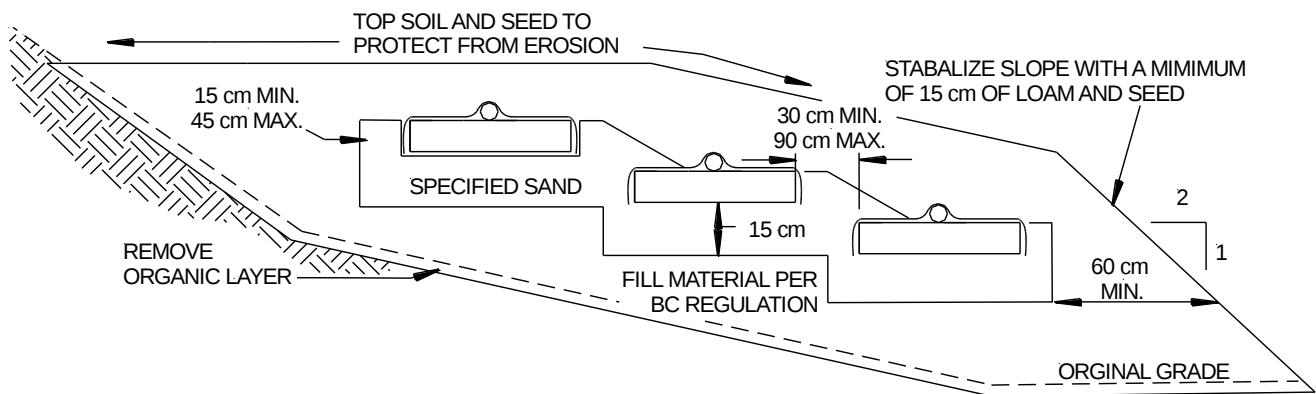
FIGURE 13: RAISED BED ON SLOPE
