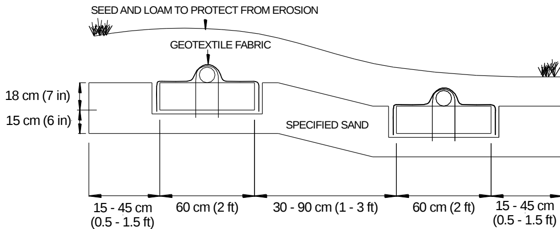
FIGURE 11: SECTION VIEW – 2 LATERAL BED SYSTEM; SLOPING SITE
