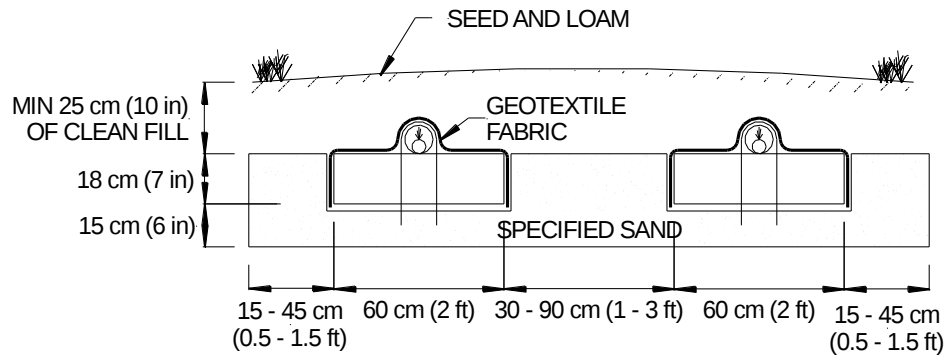
FIGURE 10: SECTION VIEW – BED SYSTEM EXAMPLE
