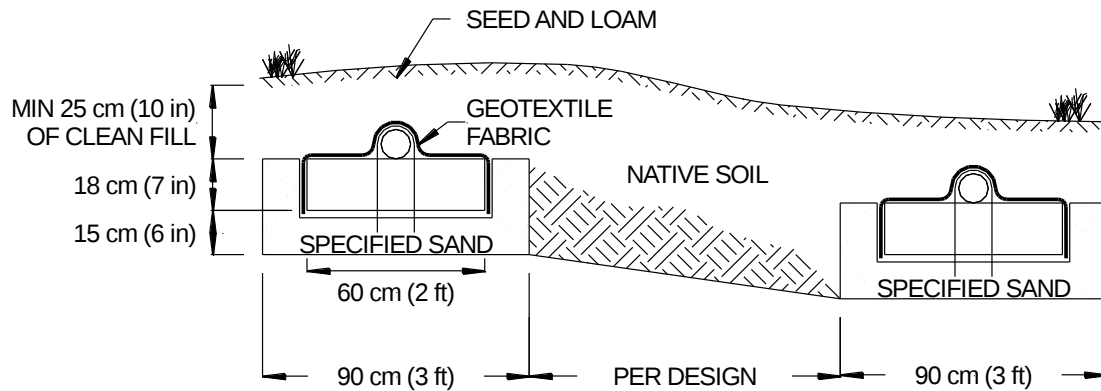
FIGURE 9: SECTION VIEW – TRENCH SYSTEM – SLOPING SITE
