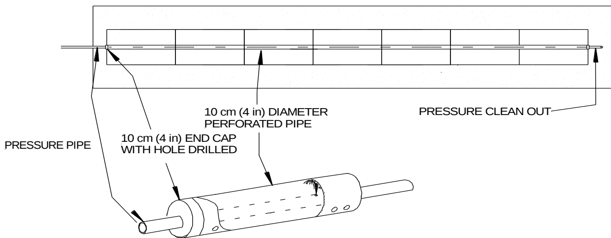
FIGURE 14: PRESSURE PIPE PLACEMENT
