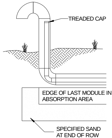
FIGURE 18: VENT LAYOUTS FOR LOW PRESSURE SYSTEMS
