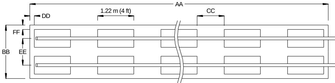
FIGURE 6: PLAN VIEW FOR WORKSHEET – TWO LATERALS
