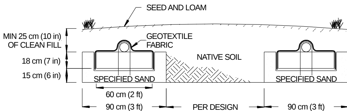
FIGURE 8: SECTION VIEW – TRENCH SYSTEM – MULTIPLE LATERALS
