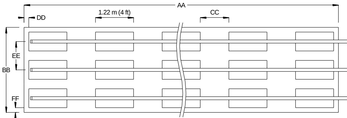
FIGURE 7: PLAN VIEW FOR WORKSHEET – THREE LATERALS
