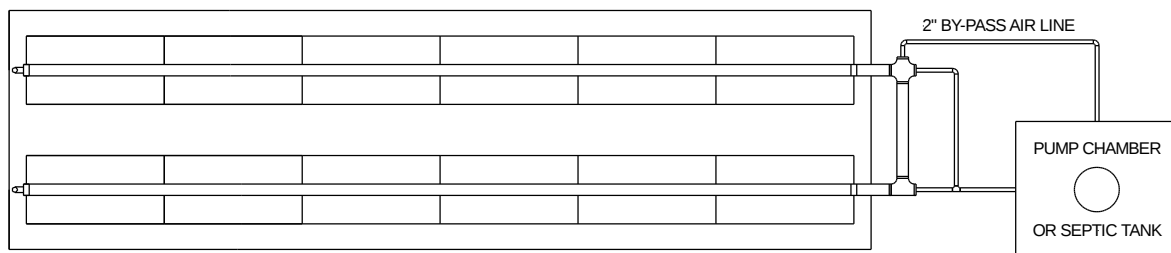
FIGURE 17: AIR BY-PASS LINE DETAIL FOR VENTING OF PUMPED SYSTEMS (WHEN REQUIRED)
