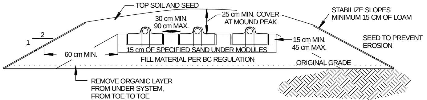
FIGURE 13: RAISED BED ON SLOPE
