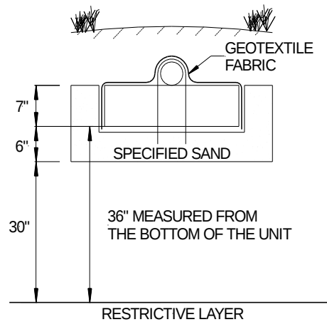
FIGURE 4: VERTICAL SEPARATION DISTANCE
