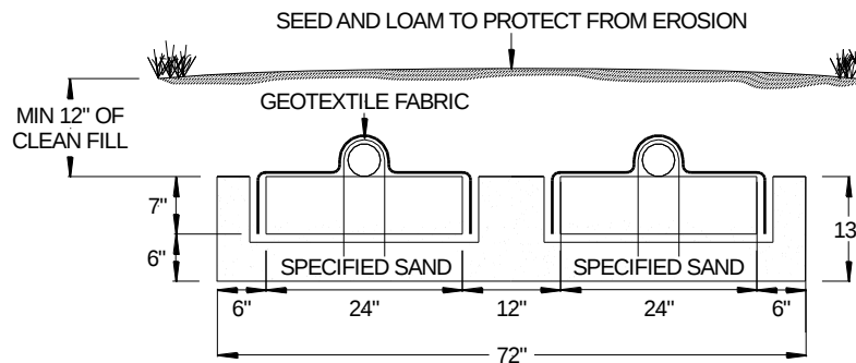
FIGURE 5: A42 DUAL LATERAL IN-GROUND CROSS SECTION
