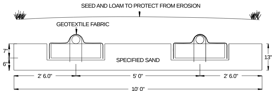
FIGURE 12: SECTION VIEW – 2 LATERAL BED SYSTEM
