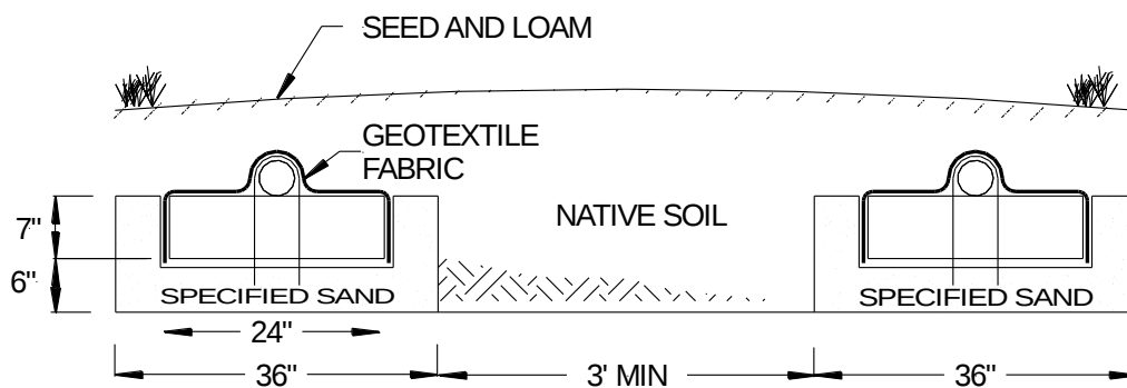
FIGURE 8: SECTION VIEW – TRENCH SYSTEM – SLOPING SITE
