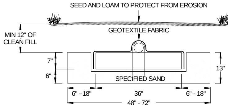
FIGURE 3: B43 TRENCH CROSS SECTION
