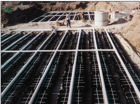
Large commercial Eljen GSF system
