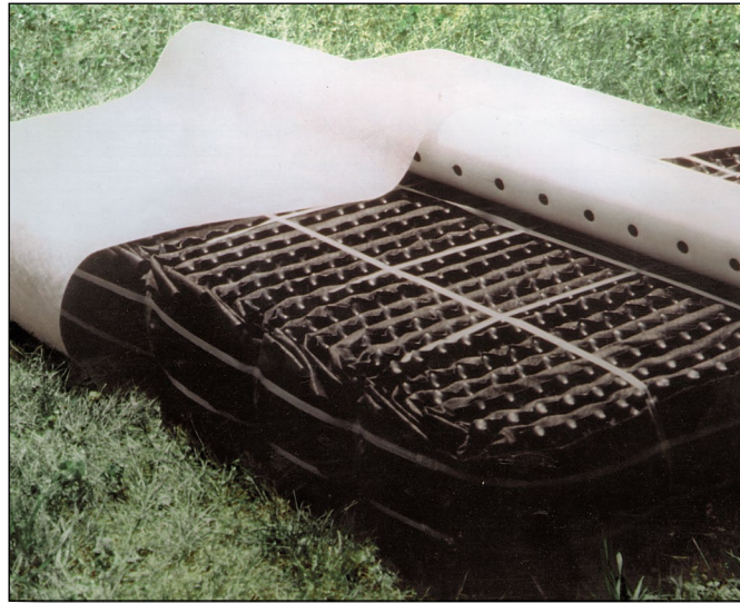
Geotextile Sand Filter Modules with pipe and geotechnical fabric
